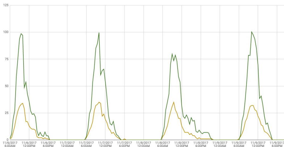
Figure 1.2: Peak kW usage and number of active charge stations.
