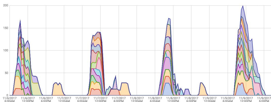
Figure 1.1: Total amperage accumulated from each charge station. Peak demand only exceeds 150 Amps of the 250 Amps available.
