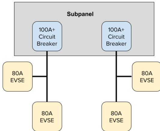
Shared Circuits
