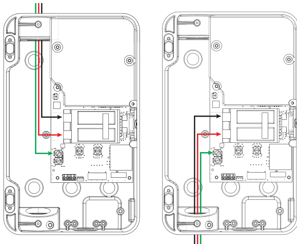
Top-Wired Install
