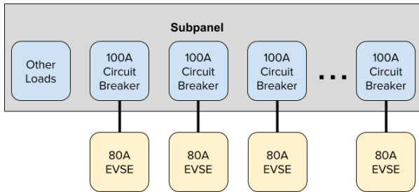
Dedicated Circuits
